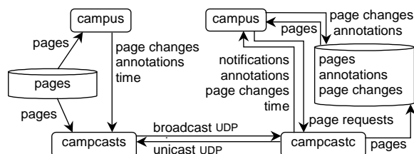
Figure 3: information flows in CORAO
