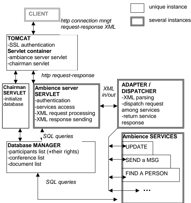
Figure 6 Server Architecture
